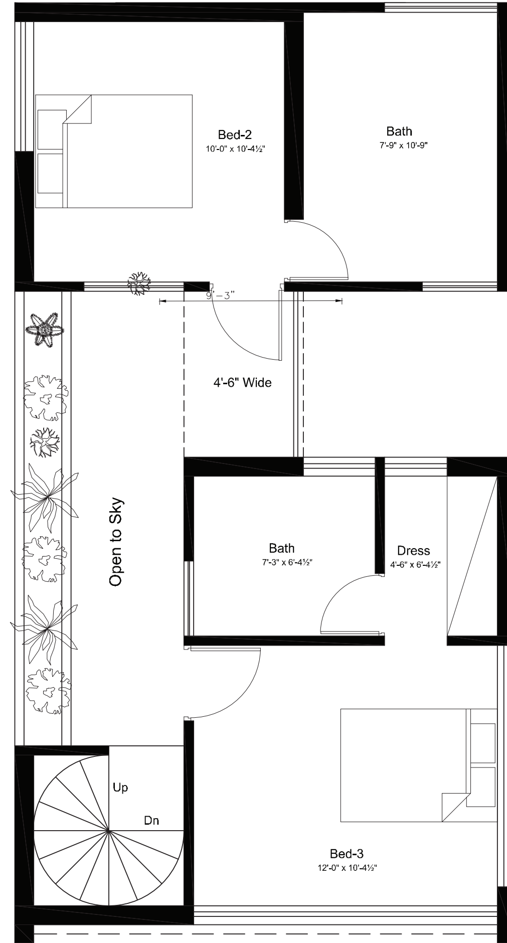
First Floor
